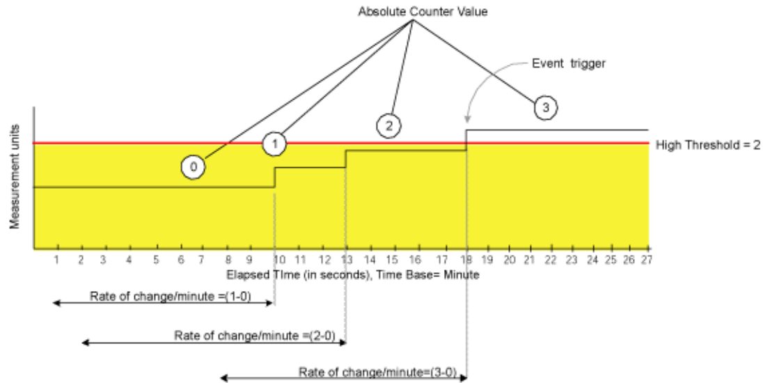
FIGURE 3 Event trigger
