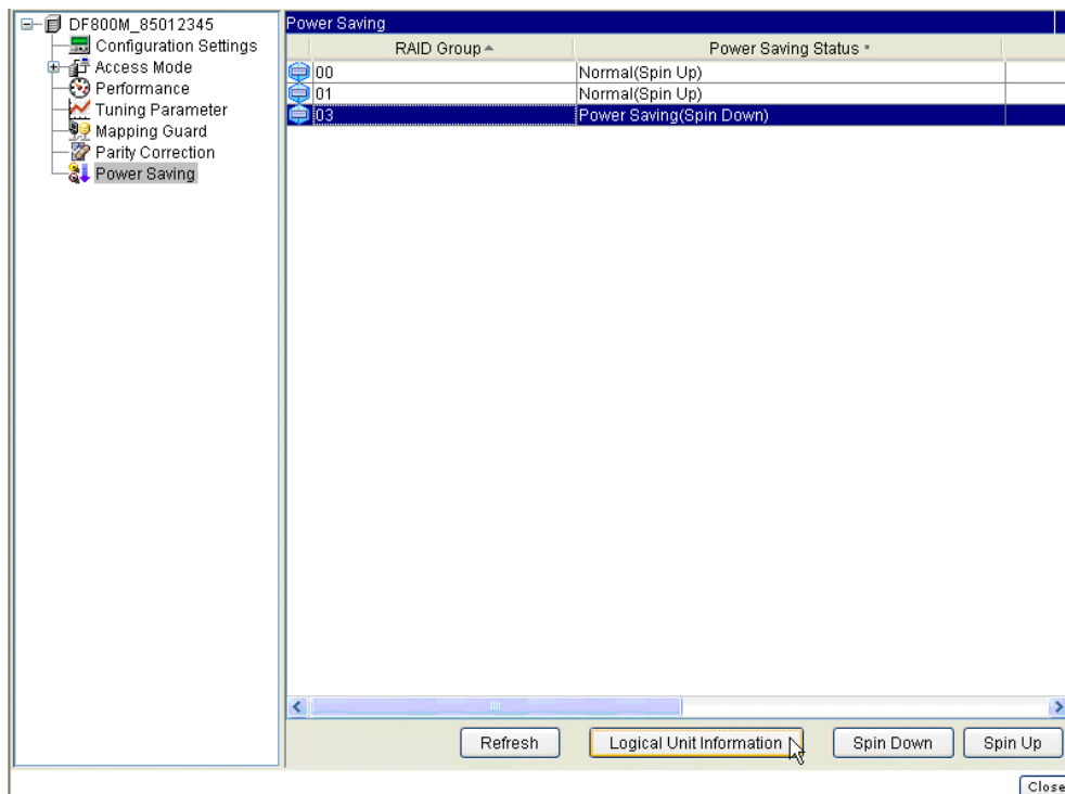
Figure 4-8: Array System Viewer
